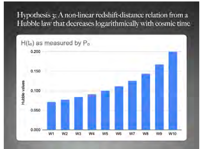
Figure 6 – A dynamic Hubble law viewed by the astronomer on W_i . Hubble's law decreases at a rate of inverse cosmic time and so the redshift-distance relation increases exponentially the farther back in time we look as well.
