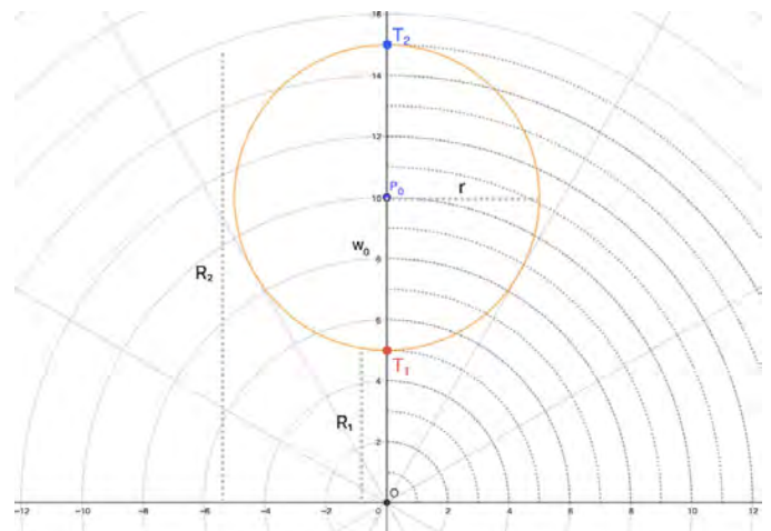
Figure 9 – Density gradient schematic of the local Big Bang Universe. Here \rho_1 and \rho_2 are at the same points as T_1 and T_2 respectively.
