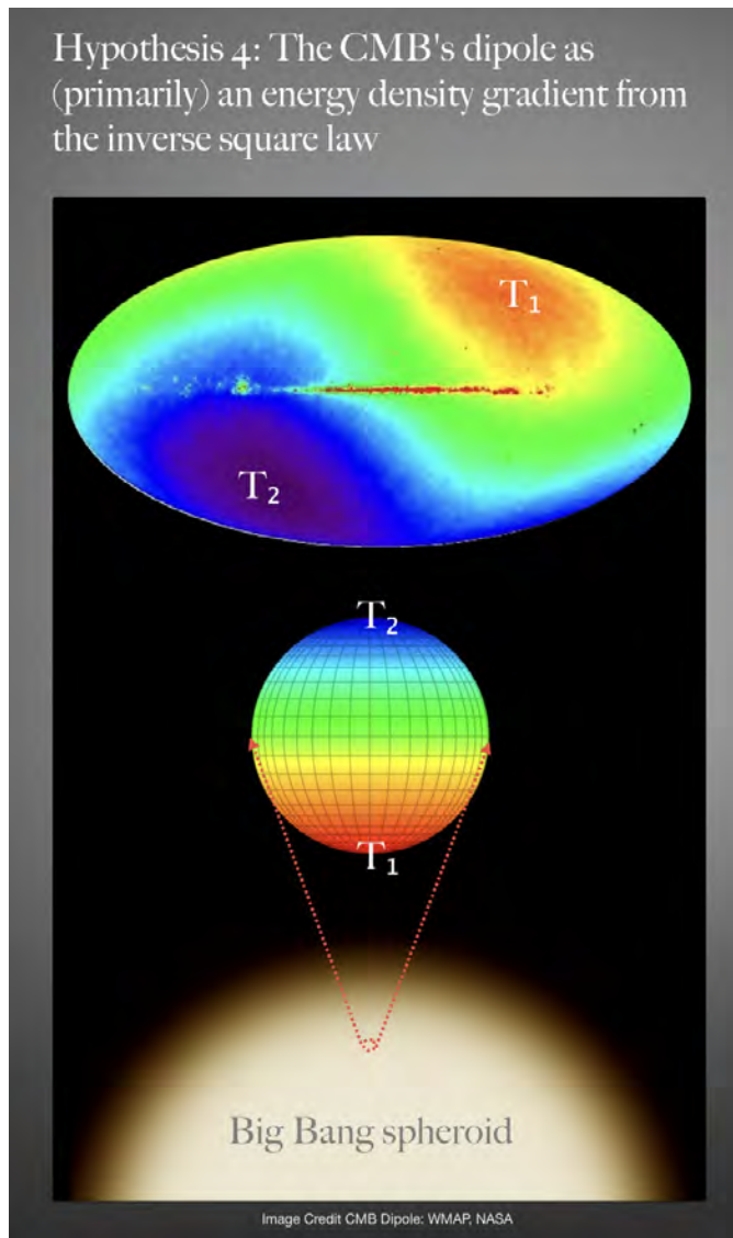
Figure 8 – The temperature dipole of the CMB were it to be a density gradient from an explosion model. The hot spot is T_1 and the cold spot is T_2 . Both an "internal" and "external" view of the dipole is shown as well as its orientation relative the Big Bang.
