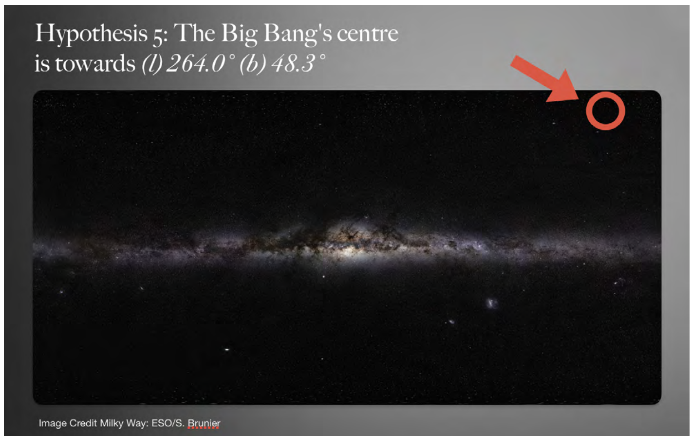
Figure 10 – The direction toward the centre of the Big Bang, according to the ALIVE model, is (l) 264.0°, (b) 48.3° in galactic coordinates.
