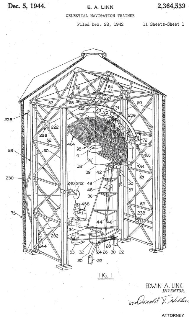
Figure 3 – Part of Edwin Link’s Patent Application for a Celestial Navigation Trainer. From Popular Science . https://patents.google.com/patent/US2364539
