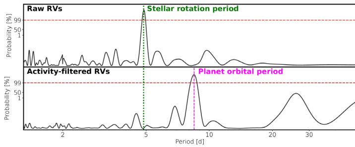
Figure 2 — These curves depict the probability of a periodic oscillation to be present in the SPIRou radial velocity (RV) data, for wobble periods ranging from 1 to 50 days. Once the periodic RV signal induced by the activity of the rotating star (at a period of 4.86 days) is corrected for in the raw RV data (upper panel), the periodic signal induced by the newly detected orbiting planet (at a period of 8.46 days) clearly shows up in the filtered RV data (lower panel) at a confidence level higher than 99.9%. Image credits: B. Klein
