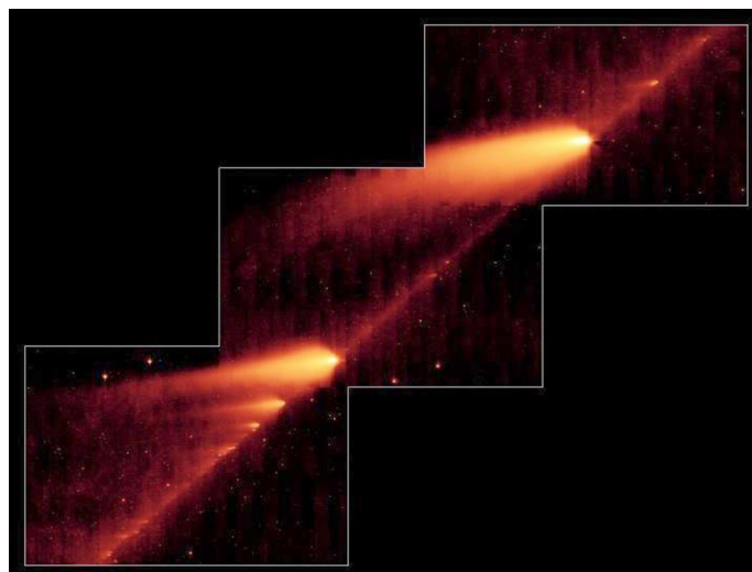
Figure 1 — Recorded on 2006 May 4-6 by the Infrared Array Camera (IRAC) on board the Spitzer Space Telescope, this image captures about 45 of 58 alphabetically catalogued large comet fragments. The brightest fragment at the upper right of the track is Fragment C. Bright fragment B is below and left of centre. Spitzer's infrared view also captures the trail of dust left over as the comet deteriorated during previous perihelion passages in 1995 and 2001. Emission from the dust particles warmed by sunlight appears to fill the space along the cometary orbit. Image credit: NASA, JPL, Caltech.
