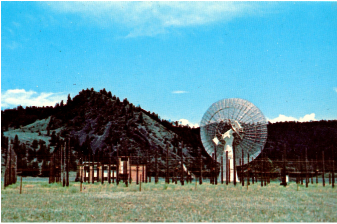
Figure 6 — The Dominion Radio Astrophysical Observatory (1960, now part of the Herzberg Astronomy and Astrophysics Research Centre), in Penticton, as it appeared in a postcard from the 1960s. The DRAO is in its turn an offspring of the DAO. Reproduced courtesy of the Specula astronomica minima .
