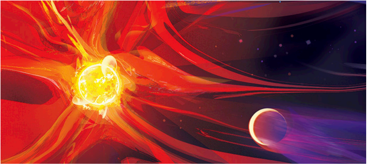
Figure 1 – Artist view of the very young eruptive red dwarf AU Mic (left) and its newly discovered close-in planet (right) with the debris disk from which the planet was born in the background. Image credits: NASA-JPL/Caltech
