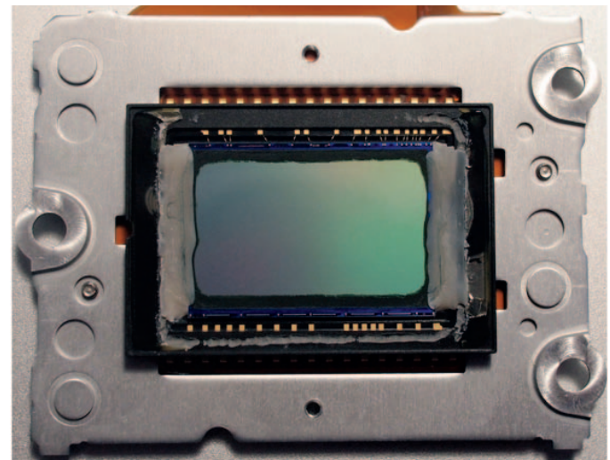
Figure 5 – Appearance of first successfully stripped D40 Sensor.
