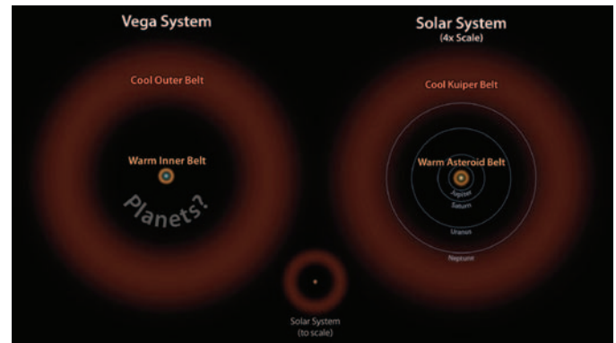
Figure 4 — Asteroid belt around the bright star Vega, as illustrated here, left, in brown.
