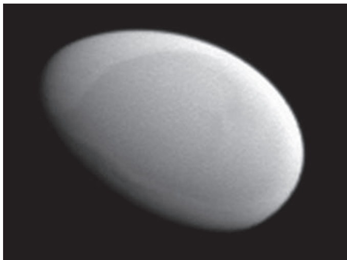
Figure 3 — Saturn's moon Methone, seen here during a Cassini flyby of the small moon on 2012 May 20.
