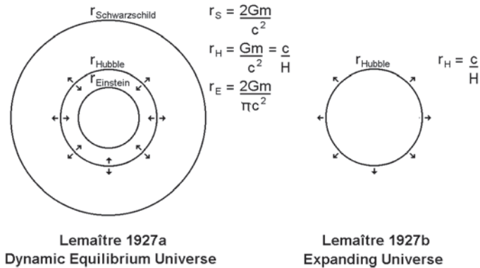
Figure 2 — Two theories of the Universe: one nearly lost to modern physics (1927a), and one that forms the basis of today's standard cosmological model (1927b).
