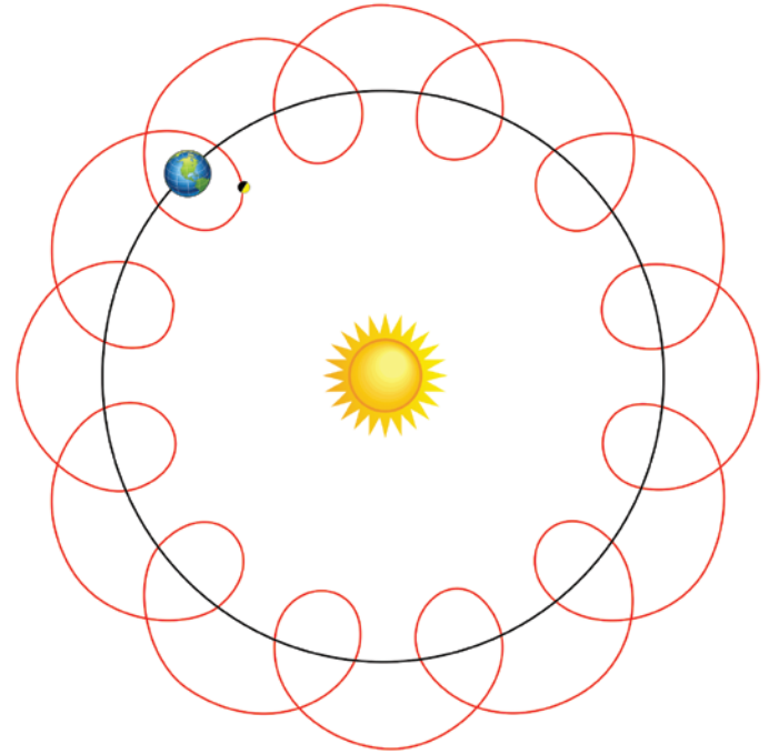
Figure 1 — It is a frequent misconception that the orbit of the Moon around the Sun forms a series of loops with the Earth at its centre.
