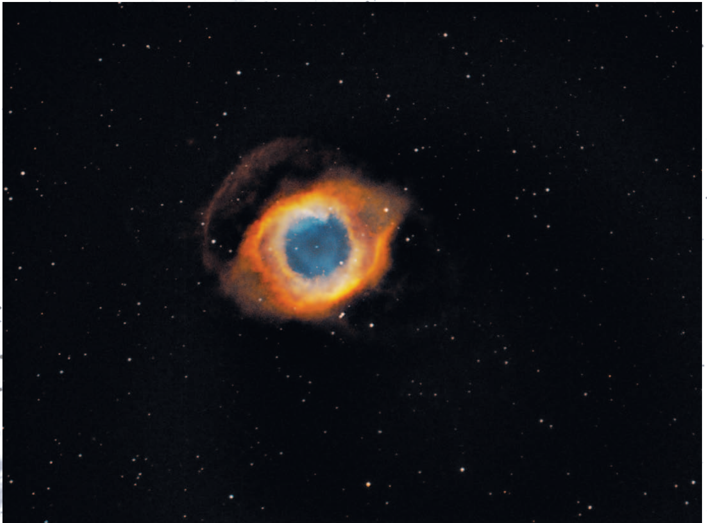
Figure 3 — Dalton Wilson captured this colourful image of the Helix Nebula (NGC 7293) last August from his observatory at Didsbury, Alberta. Dalton used an AstroTech 8" Newtonian, a QSI 583WS camera, and Astrodon H \alpha and OIII filters. Exposure in the two filters totalled nearly 7 hours. The Helix Nebula lies at a distance of 522 light-years in Aquarius.
