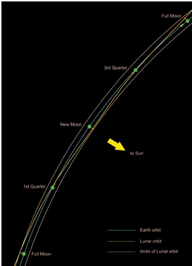
Figure 2 — The actual orbit of the Moon is similar to this schematic (it is not possible to draw a continuously concave orbit at this scale).
