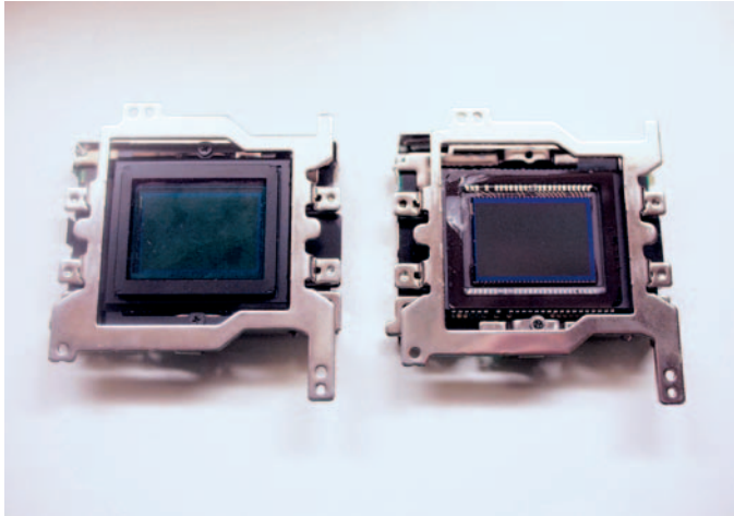
Figure 3 – Canon 10D CMOS sensors with ICF and AA filters, and without.
