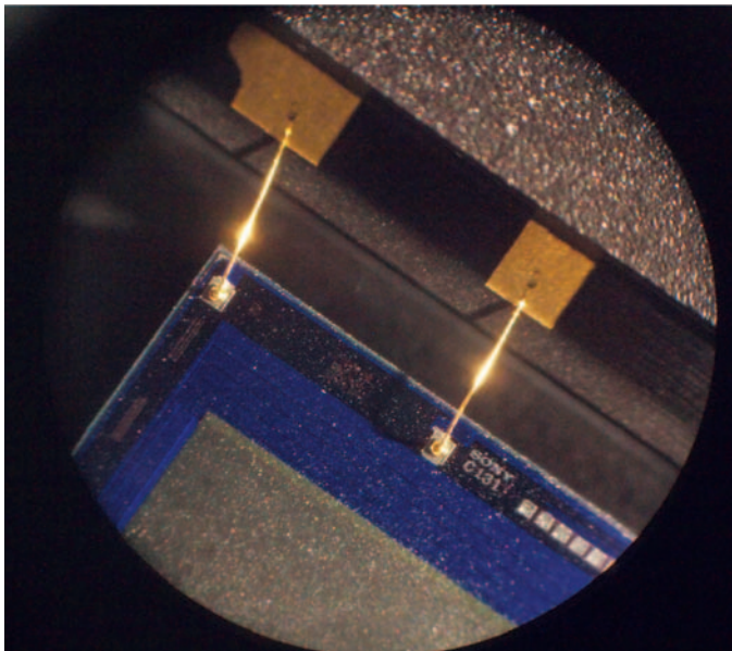
Figure 6 — Fragile gold connecting wires on D40 CCD sensor at 100× magnification.
