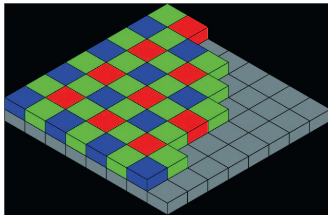
Figure 1 — Bayer Layer revealed, ubiquitous in 21st-century technology.
