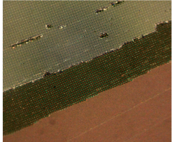
Figure 4 – 100 \times magnification image of Nikon D40 sensor surface.
