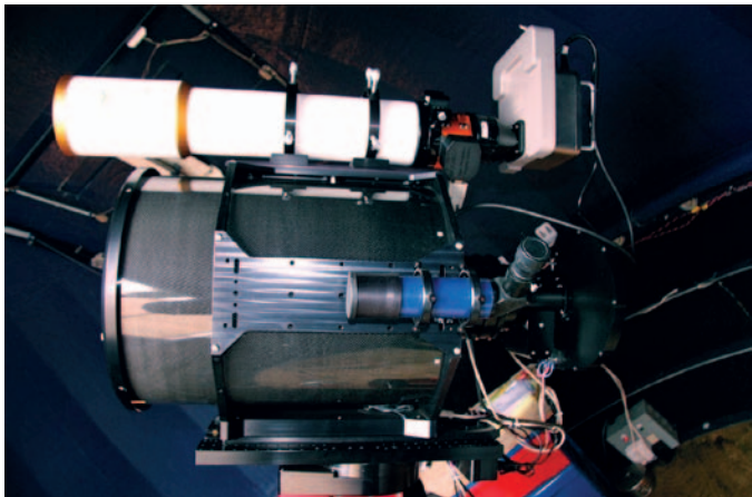
Figure 2 – The 14-inch Ceravolo Astrograph is outfitted with internal heaters and all the right stuff for a long night of imaging.
