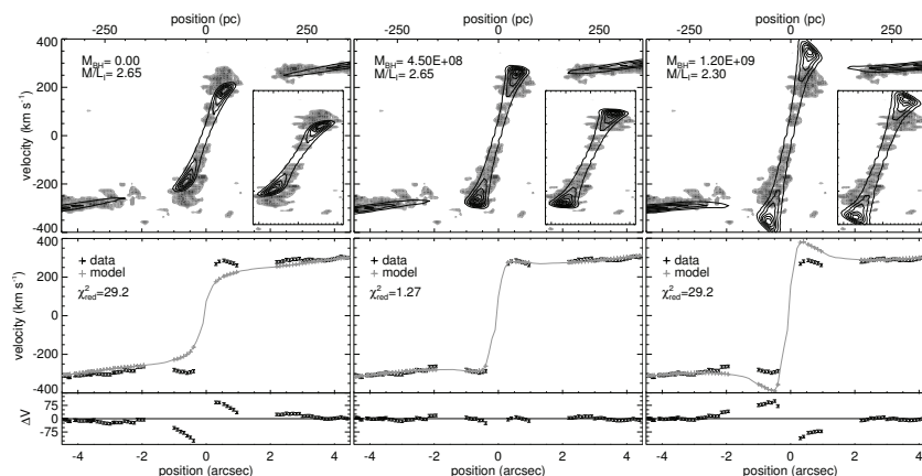
Figure 1 — In the upper three panels, the model position-velocity diagrams are shown with the black contours, while the CARMA data are in grayscale. In the lower three panels, the “residuals” (data minus model) are shown. The panels show the model with no black hole (left), the best fit (centre), and black-hole mass of 1.2 billion M_{\odot} (right). Figure courtesy of T. Davis and Nature.
