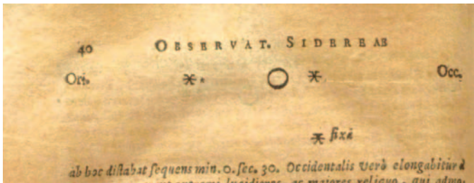
Figure 2 — This is the very last observation in Sidereus Nuncius. The star is shown just to the west of Jupiter. Opere di Galileo Galilei (1656), vol. 2, p.40; courtesy of the Thomas Fisher Rare Book Library, University of Toronto.
