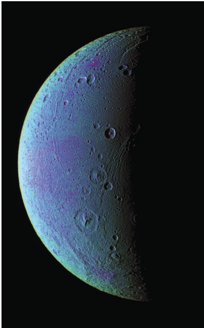
Figure 2 — January 2006 false-colour view highlights tectonic faults and craters on Dione, an icy world. Oxygen ions are sparse—one for every 11 cubic centimetres of space or about 90,000 per cubic metre. Dione has an extremely thin neutral atmosphere.
