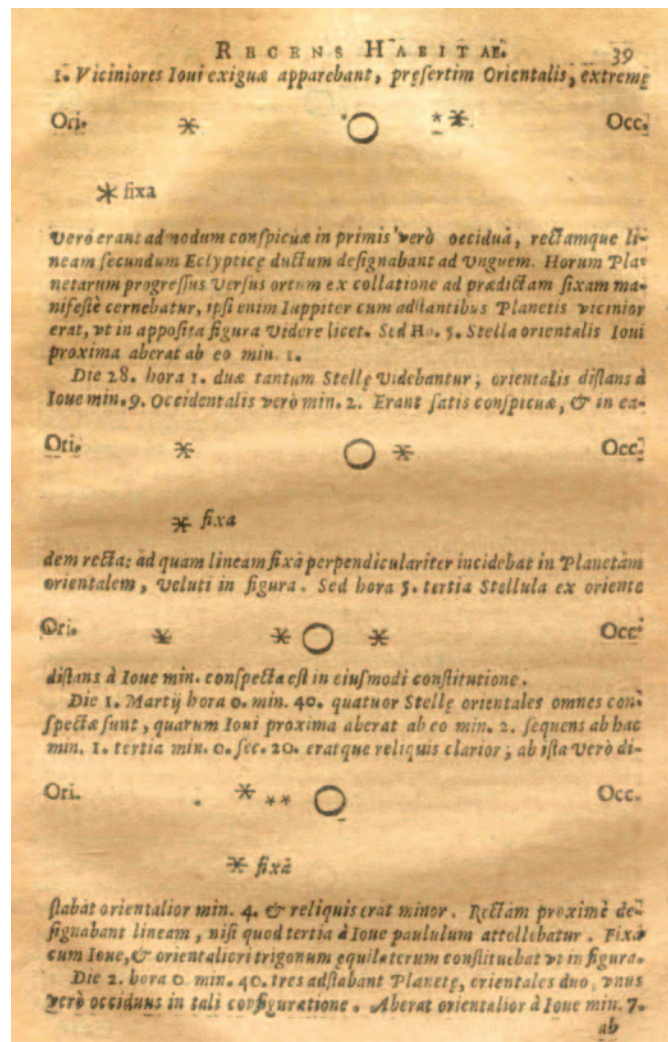
Figure 1 — Galileo's sketches and notes published in Sidereus Nuncius . 1610 February 27, 28, and March 1 clearly illustrate the night-to-night eastern progression of Jupiter and its moons. Opere di Galileo Galilei (1656), vol. 2, p.39; courtesy of the Thomas Fisher Rare Book Library, University of Toronto.
