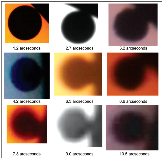
Figure 1 – Photographs of the black-drop effect during the ToV of 2012, taken by the SDO, Y. Tremblay, M. Savoie, F. Tomaras-1, M. Brault, R. Sauv , A. Gendron (ToV of 2004), J.M. Gohier, and F. Tomaras-2, respectively from left to right and top to bottom. The resolution of the telescopes used is indicated in arcseconds, as deduced from the width of the halos around Venus and the Sun.
