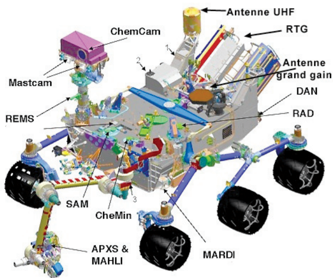
Figure 2 — Curiosity rover
