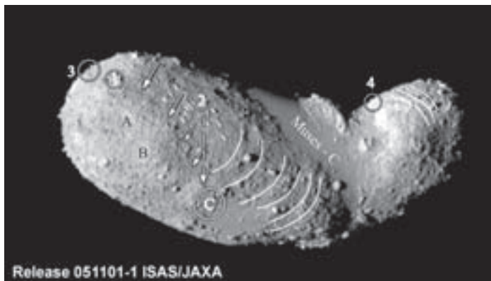
Figure 1 — Boulder mounds (1, 2, 3, and 4) with debris-flow levees following a course from (1) marked with solid arrows, ending at C. The mass-wasted feature is ~250 m in length with the levees visible on the available lower-resolution imagery. The boulder mound at (2) leads into a series of parallel channels that could either contain debris flows, which are beyond the resolution of the image, or are catchments that have directed meltwater toward sink C. Craters are the lighter areas marked A and B, presumably of a young age as depicted by lack of space weathering and retention of rim form. Lobate-shaped forms of pseudo-stone-banked lobes are delimited with parabolic curves to the right of the channels and to the left of the Muses-C area — a large depression infilled with fine gravel and sand, nearly devoid of large clasts. To the right of the Sea of Muses, the light-coloured channels, oriented north-south, originate in a mound of boulders at the top of the image, and may well mark meltwater release flooding to the south. Clast orientation similar to talus on Earth is shown with white lines oriented to southeast. Source: 051101-1 ISAS/JAXA.
