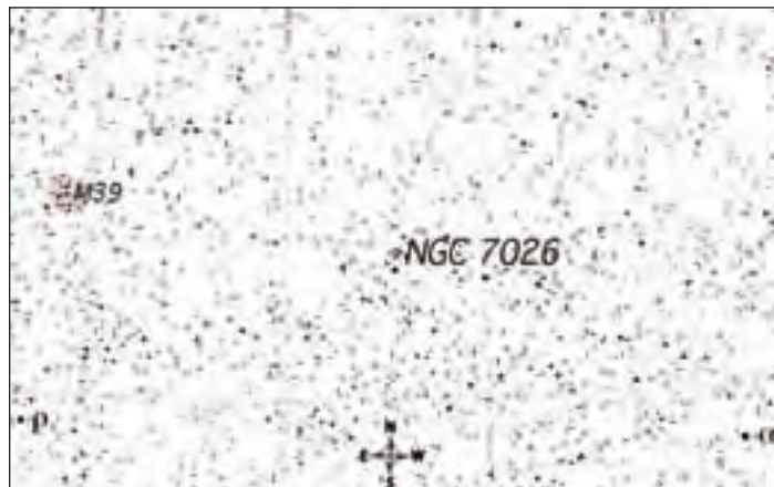
Figure 2 — Finder chart for NGC 7026.
