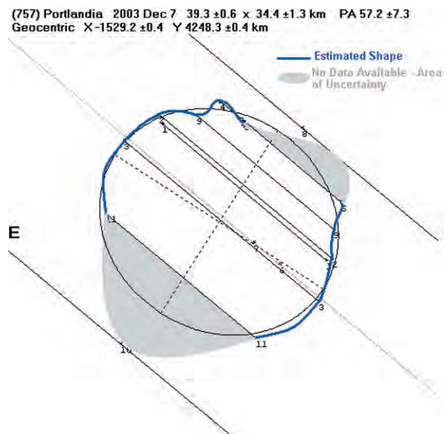
Figure 1 – Sky-plane plot for the December 07, 2003 occultation by asteroid (757) Portlandia of the star HIP 384. Eight observers’ chords are plotted, but only a very rough shape and size of the asteroid can be inferred. More observers, particularly in the grey regions, would have helped define the shape and resolution of the profile.
