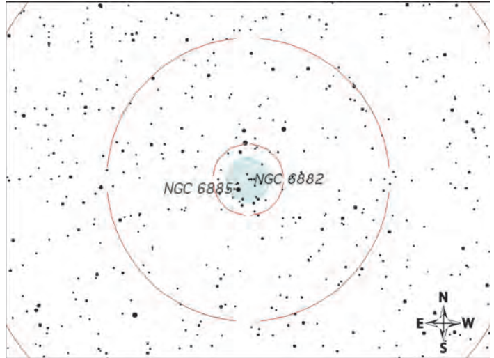
Figure 2 – Finder chart for NGC 6882/6885 shown with 0.5° and 2° Telrad circles (and part of 4° circle).
