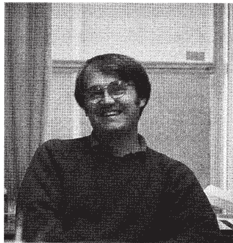
David Clarke is a radio astronomer who studies plasma clouds
