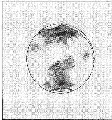
Mars as drawn by Murray Paulson on Jan. 24, 1995. He used 540x on a 12.5" with a 7mm Nagler and 2.4x Barlow. Seeing was rated 6.
