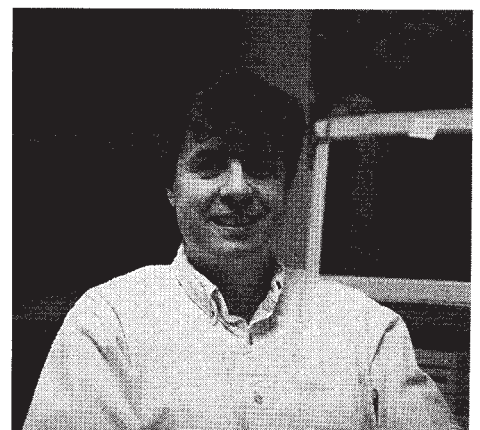
David Guenther probes the conditions within stars
