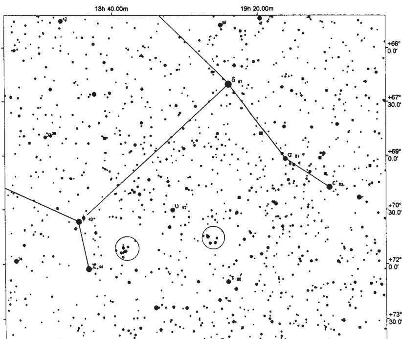
The constellation Draco includes two asterisms (circled) that resemble Cassiopeia (left) and a hoard of diamonds (right). Chart by permission of MegaStar.
