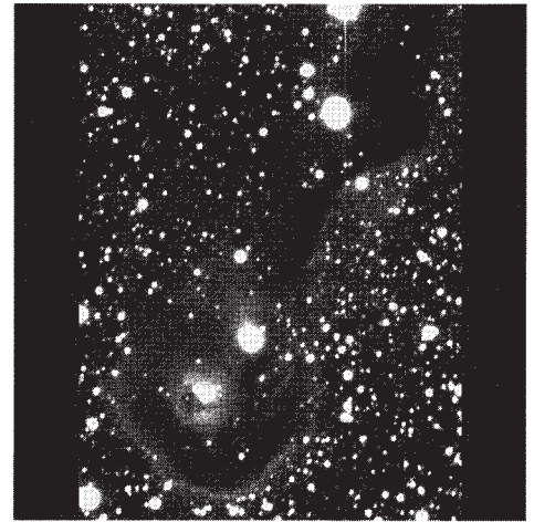
A 464-minute exposure by Paul Boltwood of vdB 142 within the nebula IC 1396. The image covers 8.8 by 13.2 arcminutes.
